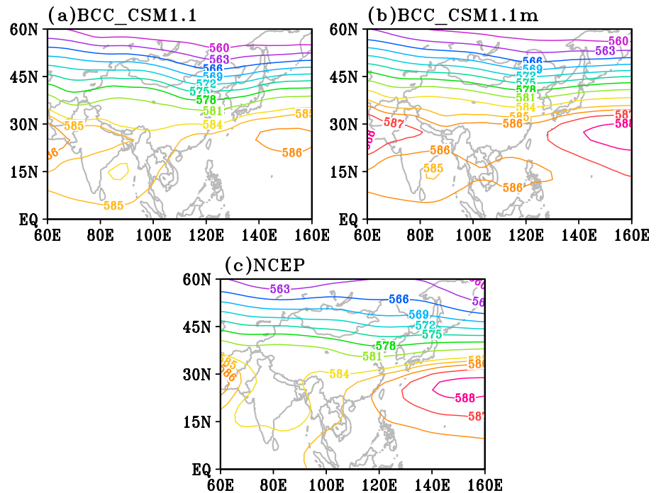
Figure 11. The modeled and NCEP reanalysis summer geopotential height at 500 hPa level averaged over 1960–2012 (unit: dgpm).
