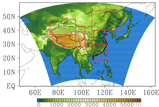
Figure 3. The surface elevation on each model grid in the model domain. The nine subregions are denoted by red rectangles (a = Reg1, b = Reg2, c = Reg3, d = Reg4, e = Reg5, f = Reg6, g = Reg7, h = Reg8, and i = Reg9). The gray line marks the elevation of 3,000 m.
